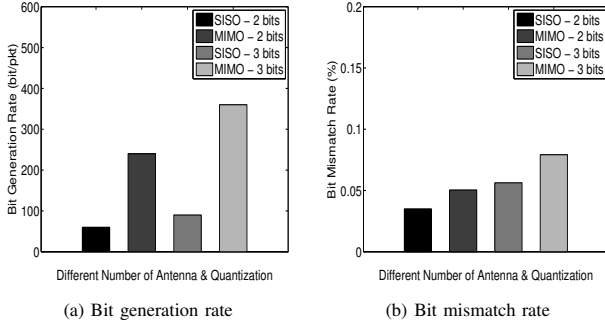
Fig. 8. Performance of CSI based method when exploiting MIMO system.
