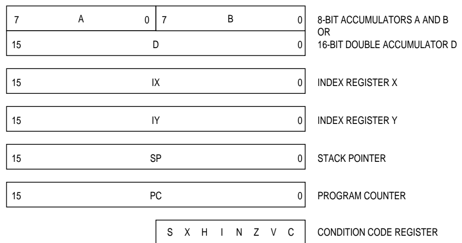
Figure 2-1. Programming Model
