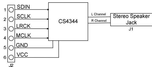
Block Diagram
