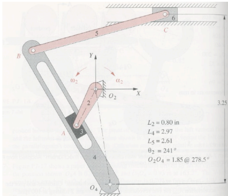
Figure 1. Slider Mechanism. (Norton, 3 rd Edition, pg 368)
