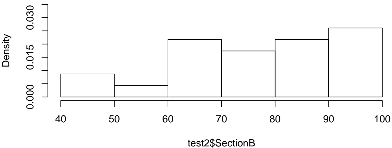
Histogram of test2$SectionB
