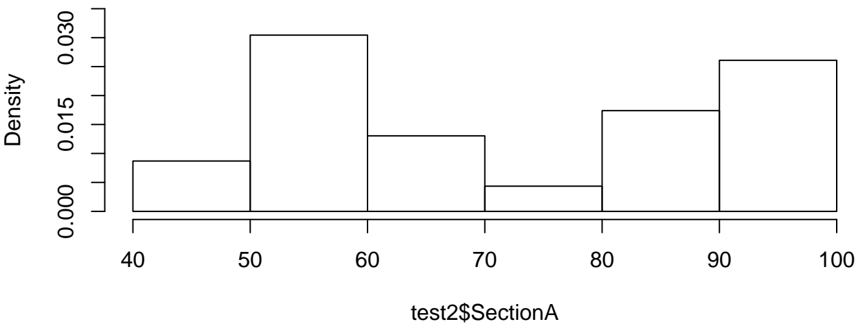
Histogram of test2$SectionA
