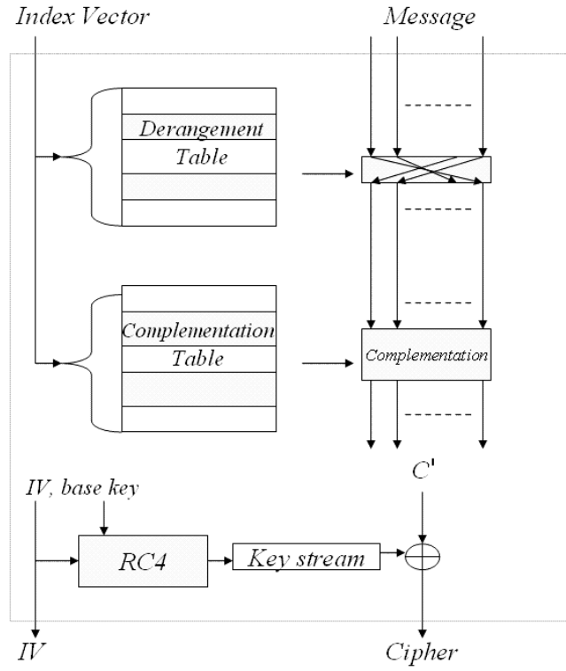
Fig. 1. Block diagram of the proposed LWE scheme
