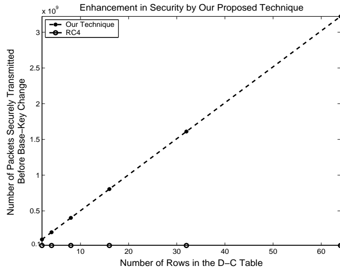
Fig. 2. Enhancement in security due to the proposed LWE for a 128 bit message length and 104 bit RC4 base key
