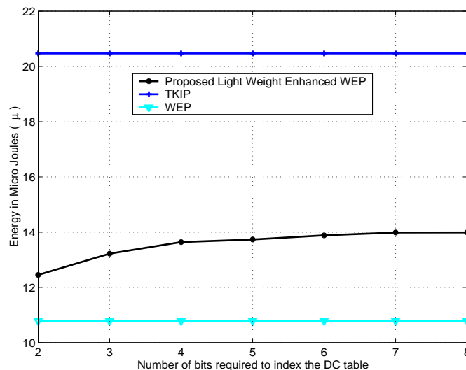
Fig. 4. Energy consumption per 256 byte frame by WEP, TKIP, and the proposed light weight enhanced WEP against different sizes of the D-C table used in our proposed technique.
