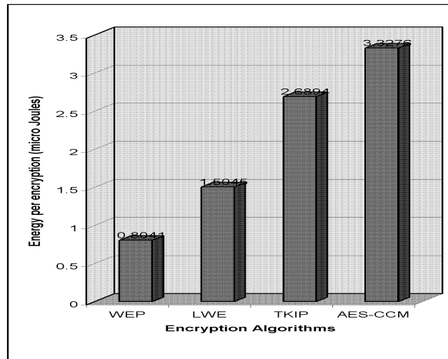
Fig. 5. Energy consumption per encryption by WEP, TKIP, proposed Light Weight Enhanced WEP (LWE) and AES-CCM protocol.
