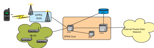
Figure 1: Tight coupling architecture for GPRS integrated with Wi-Fi networks.
