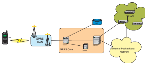
Figure 2: Loose coupling architecture for GPRS integrated with Wi-Fi networks.
