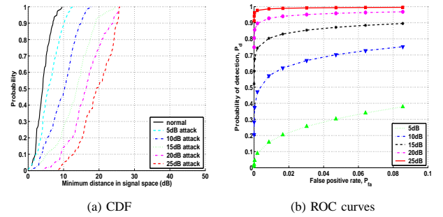
Fig. 5. CoRE 802.11: (a) Cumulative Distribution Function (CDF) of minimum distance D_s in signal space. (b) Minimum distance D_s : Receiver Operating Characteristic (ROC) curves
