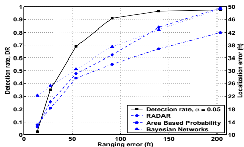
Fig. 13. CoRE 802.11: Relationships among Detection Rate (DR), ranging error, and localization error.
