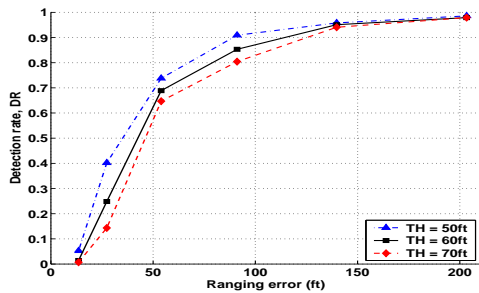
Fig. 8. CoRE 802.11, NLS using \mathcal{E} : effectiveness of attack detection
