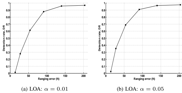
Fig. 4. CoRE 802.11, LLS residuals: effectiveness of attack detection
