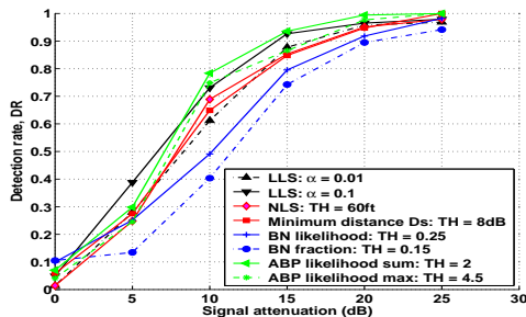
Fig. 12. CoRE 802.11: Comparison between generic and specific test statistics for attack detection.
