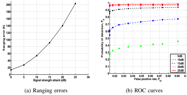
Fig. 3. CoRE 802.11: (a) Ranging errors under the signal strength attacks (b) LLS residuals: Receiver Operating Characteristic (ROC) curves
