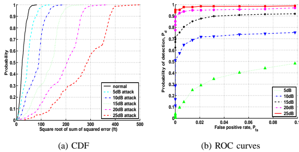
Fig. 7. CoRE 802.11, NLS: (a) Cumulative Distribution Function (CDF) of \mathcal{E} . (b) \mathcal{E} : Receiver Operating Characteristic (ROC) curves
