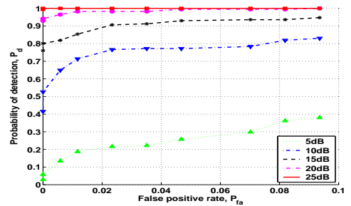
Fig. 10. CoRE 802.11, ABP: Receiver Operating Characteristic (ROC) curves
