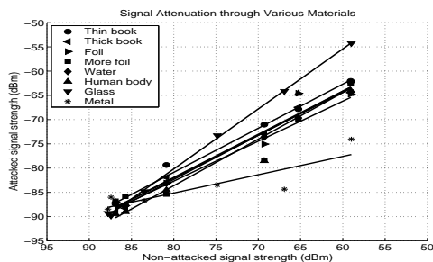
Fig. 1. Linear attack model on received signal strength for various media.
