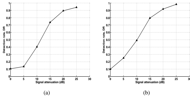
Fig. 11. CoRE 802.11, BN: (a) Using fraction of contribution of each landmark for attack detection with threshold = 0.15. (b) Using likelihood in Bayesian inference for attack detection with threshold = 0.25.
