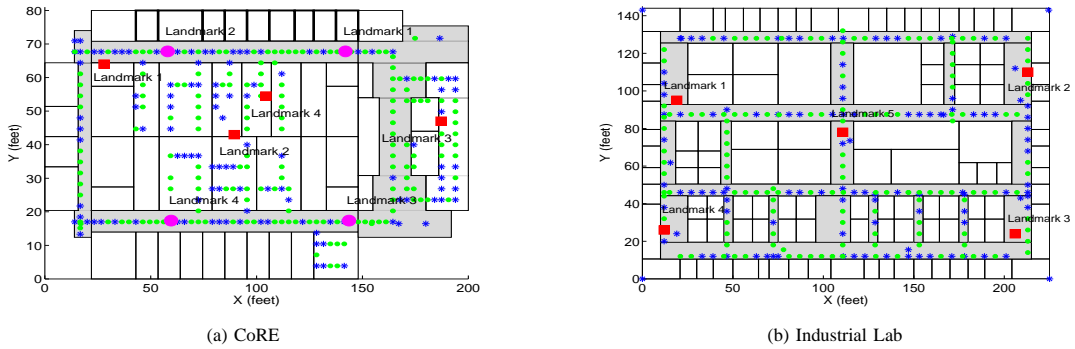
Fig. 2. Layout of the experimental floor
