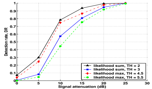
Fig. 9. CoRE 802.11, ABP: effectiveness of attack detection
