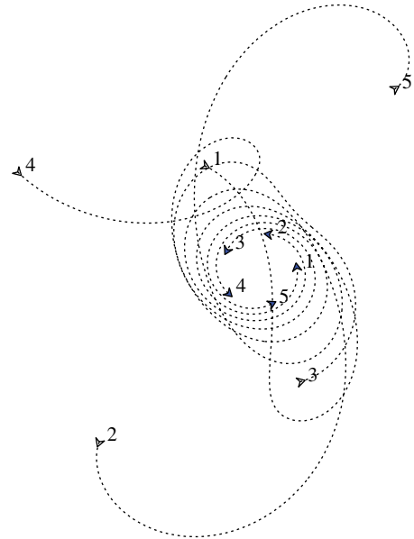
Fig. 3. Five unicycles, k_\alpha = 1 , k_r < k^* .
