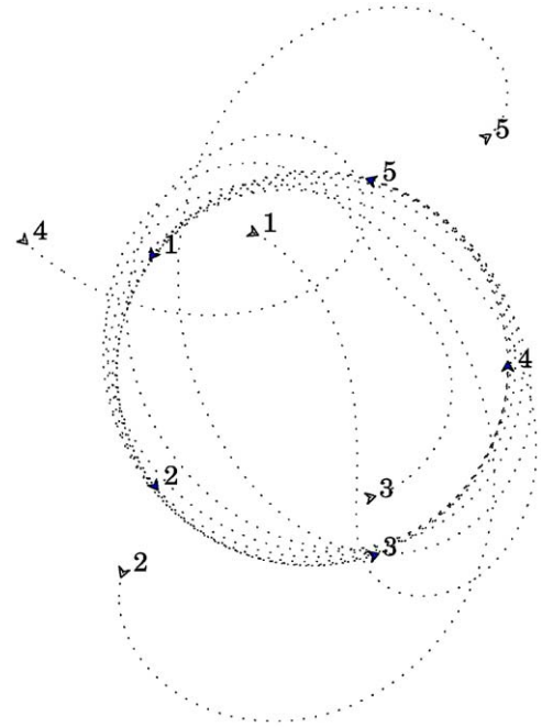
Fig. 2. Five unicycles, k_\alpha = 1 , k_r = k^* .
