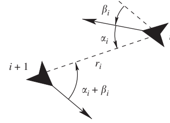
Fig. 1. New coordinates, with unicycle i in pursuit of i + 1 .
