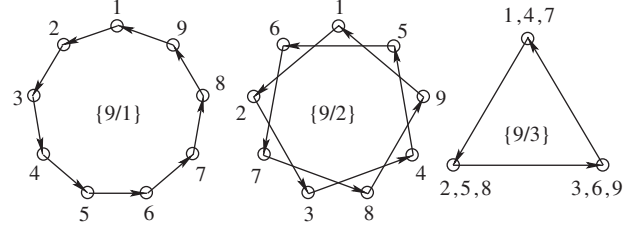
Fig. 5. Generalized regular polygons \{9/d\} , d \in \{1, 2, 3\} .
