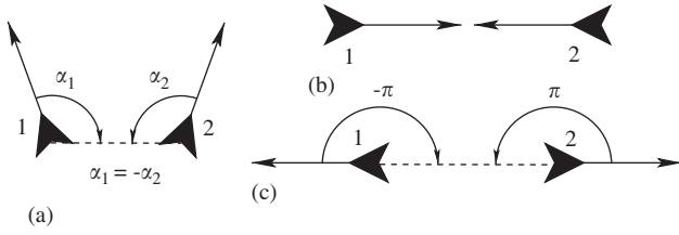
Fig. 6. Possible configurations for \xi(0) \in \mathcal{W} .
