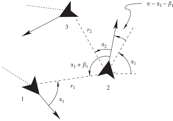
Fig. 7. Depiction of coordinates for unicycles 1 and 2.
