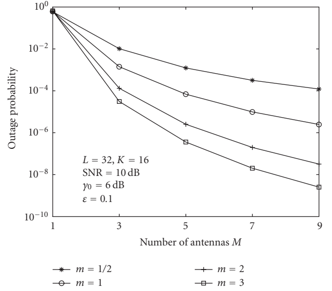
FIGURE 6: Outage probability versus number of antennas M and Nakagami m .
