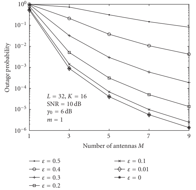
FIGURE 4: Outage probability versus number of antennas M and NFCO \varepsilon .
