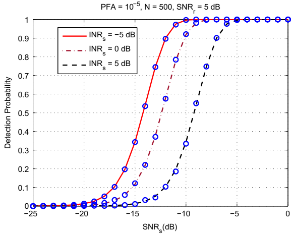
Fig. 3. Detection performance of the CC detector with different values of INR_s . The symbols “o” denote the MC results, and the lines denote the results obtained using (11).
